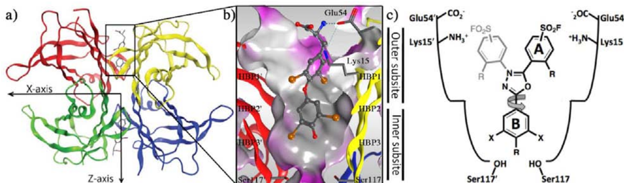
Figure 1. Structure of homotetrameric WT-TTR with a focus on the T_4 binding pocket. (a) Crystal structure of WT-TTR in complex with T_4 (2ROX). (b) Close-up view of one of the two identical T_4 binding sites showing a ribbon depicted tetramer (colored by chain) with a “Connolly” molecular surface applied to residues within 8 Å of T_4 (hydrophobic = gray, polar = purple). The innermost HBP3 and 3' are composed of the methyl and methylene groups of Ser117/117', Thr119/119', and Leu110/110'. HBP2 and 2' are made up by the side chains of Leu110/110', Ala109/109', Lys15/15', and Leu17/17'. The outermost HBP1 and 1' are lined by the methyl and methylene groups of Lys15/15', Ala108/108', and Thr106/106'. These figures were generated using the program MOE (2011.10). (c) Schematic representation of the T_4 binding pocket with both the inner/outer binding subsites labeled and the amino acids that are being targeted in the design and optimization of substituents of aryl rings A and B. Rotation around the 1,3,4-oxadiazole ring linker gives rise to the symmetry related binding mode within the symmetrical T_4 pocket.
