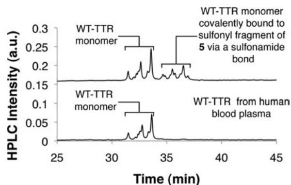
Figure 7. Example \text{C}_{18} -RP-HPLC analysis of the modification of WT-TTR (6.4 \mu\text{M} ) in human blood plasma by compound 5 (6.4 \mu\text{M} ). Several oxidized Cys10 isoforms of TTR exist in human plasma, as ascertained by liquid chromatography and/or mass spectrometry. 76–79 Cys10 makes a mixed disulfide with the amino acid cysteine (TTR-Cys), the peptide glutathione (TTR-GSH), and the peptide cysteinylglycine (TTR-CysGly) and can be oxidized to S-sulfonated TTR.
