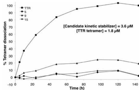
Figure 6. Influence of covalent kinetic stabilizers 5 , 9 , and 15 (3.6 \mu M) on the rate of WT-TTR tetramer dissociation relative to WT-TTR (1.8 \mu M tetramer) in the absence of a covalent kinetic stabilizer. Dissociation and unfolding of TTR in 6 M urea is monitored by far-UV CD at 215–218 nm over 144 h after a 1 h preincubation period with covalent kinetic stabilizer.
