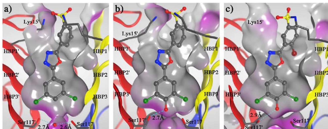
Figure 8. Crystal structures of homotetrameric WT-TTR in complex with inhibitors 9 , 5 , and 15 (panels a–c, respectively). Close-up view of one of the two identical T_4 binding sites in a ribbon depicted tetramer colored by chain. A “Connolly” molecular surface was applied to residues within 8 Å of ligand in the T_4 binding pocket: hydrophobic (gray) and polar (purple). The innermost HBPs 3 and 3' are composed of the methyl and methylene groups of Ser117/117', Thr119/119', and Leu110/110'. HBPs 2 and 2' are made up by the side chains of Leu110/110', Ala109/109', Lys15/15', and Leu17/17'. The outermost HBPs 1 and 1' are lined by the methyl and methylene groups of Lys15/15', Ala108/108', and Thr106/106'. Hydrogen bonds shown in light-blue dashed lines, with the atomic distances labeled in Å. This figure was generated using the program MOE (2011.10).
