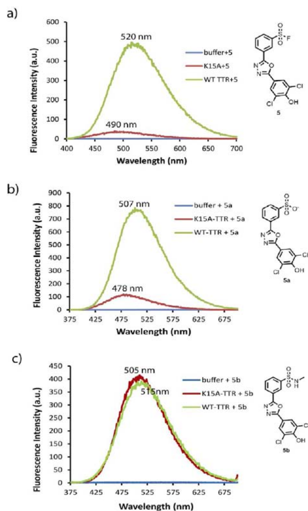
Figure 10. Fluorescence emission spectra of compounds 5 , 5a , and 5b after 18 h incubation with WT- and K15A-TTR ( \lambda_{\max \text{ ex}} for 5 , 5a , and 5b is 365, 342, and 355 nm, respectively).
