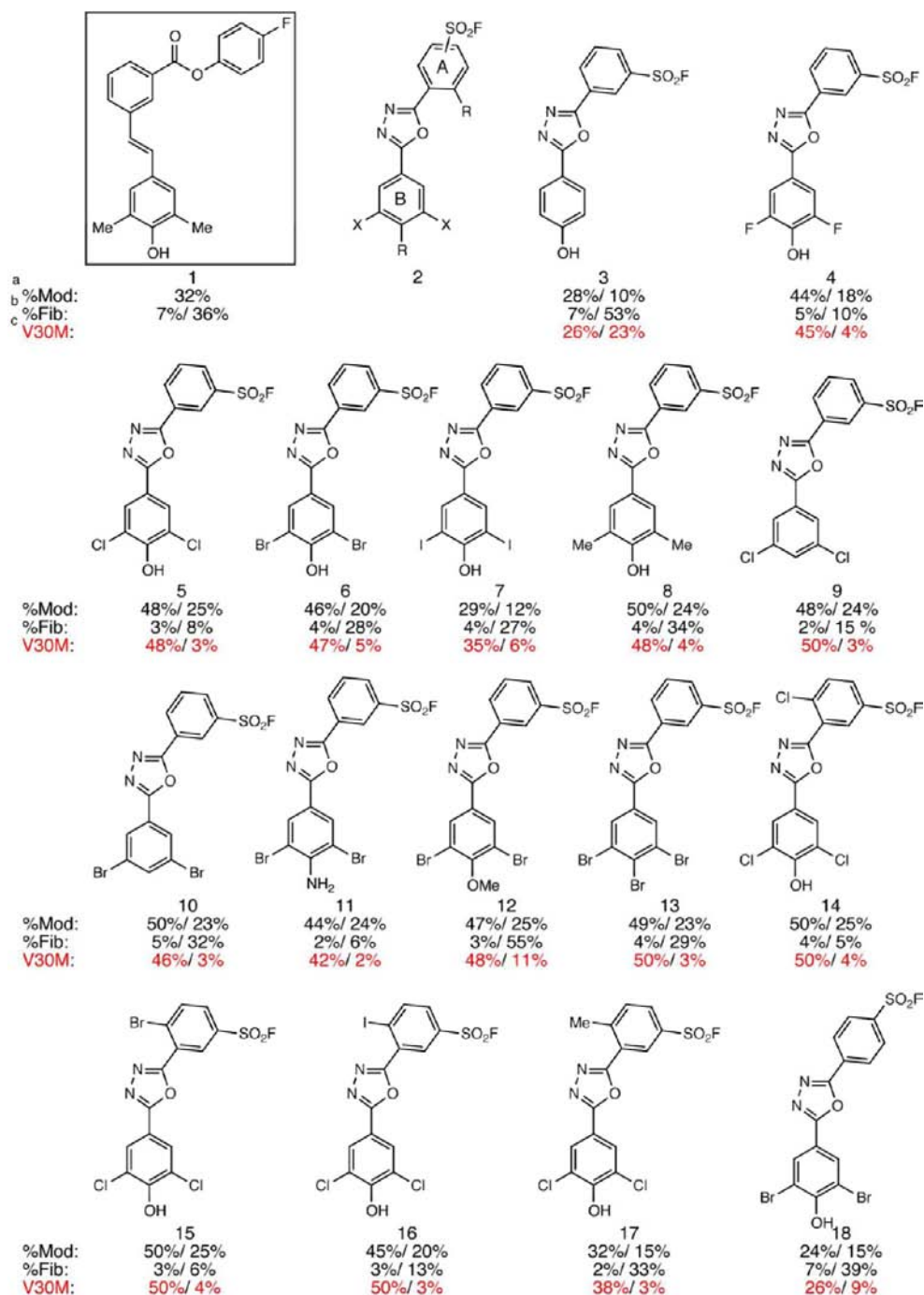
Figure 3. Library of sulfonyl fluoride containing 1,3,4-oxadiazoles. (a) Percentage modification of WT-TTR (black font) at 2:1/1:1 stoichiometries. 50% represents maximum covalent modification at 2:1 stoichiometry. (b) Percentage aggregation observed at 2:1/1:1 stoichiometries, compared to unstabilized WT-TTR (100%). (c) Percentage modification of V30M-TTR (red font) at 2:1 stoichiometry/% aggregation observed at 2:1 stoichiometry. See Table S3 for errors.
