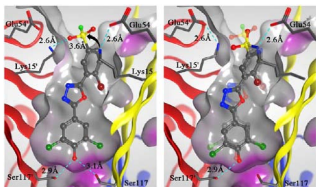
Figure 9. Structural basis for sulfonamide activation. (Left) The docked structure of 15 into the T_4 binding site showing nucleophilic attack on the sulfonamide sulfur atom from the K15 \epsilon -amino group as depicted by a black arrow. (Right) Crystal structure of homotetrameric WT-TTR as a conjugate after reaction with 15 and superposition of the unreacted docked conformation of 15 as a ghost view. Both show a close-up view of one of the two identical T_4 binding sites in a ribbon depicted tetramer colored by chain. A “Connolly” molecular surface was applied to residues within 8 Å of ligand in the T_4 binding pocket—hydrophobic (gray), polar (purple). Hydrogen bonds shown in light blue dashed lines, with the atomic distances labeled in Å. This Figure was generated using the program MOE (2011.10), Chemical Computing Group, Montreal, Canada.
