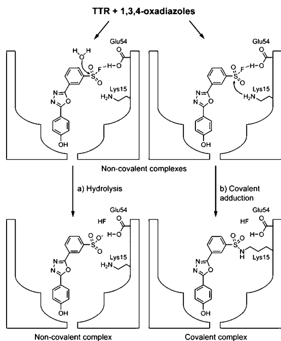
Figure 2. An illustration of the potential fates of 1,3,4-oxadiazoles in the TTR binding pocket. TTR and 1,3,4-oxadiazoles initially form noncovalent complexes. Then the functional groups on the side chains that line the binding pocket can catalyze either hydrolysis (path a) or covalent adduction (path b) by stabilization of the fluoride leaving group. We show Glu54 performing this function, but there are other possibilities, including the Glu54–Lys15 salt bridge.
